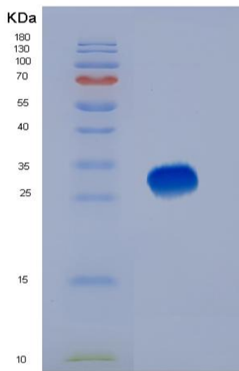
Figure 2. SDS-PAGE
