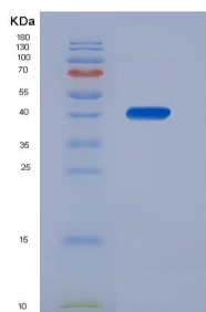
Figure 1. SDS-PAGE
